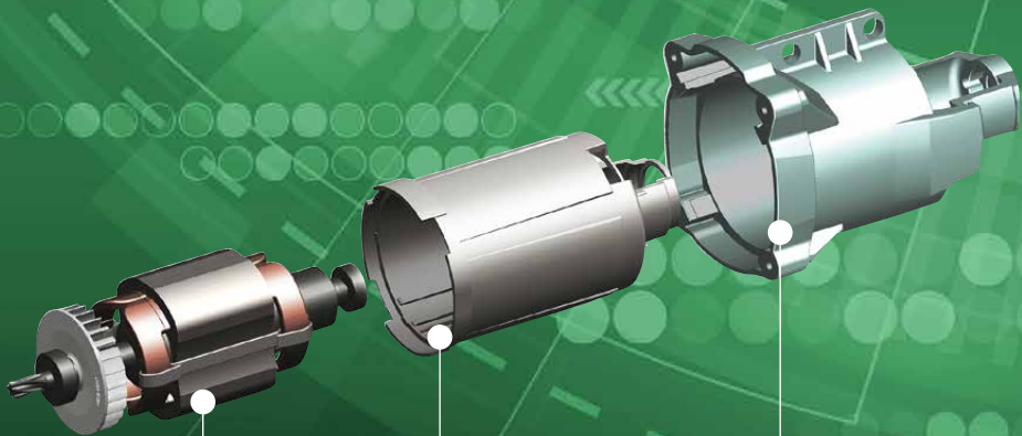
Plastic stator holder
