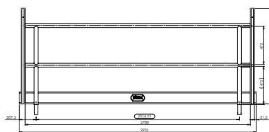
331523 Leuning MTB 3 m
