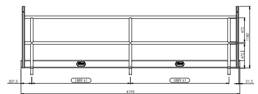
331524 Leuning MTB 4 m
